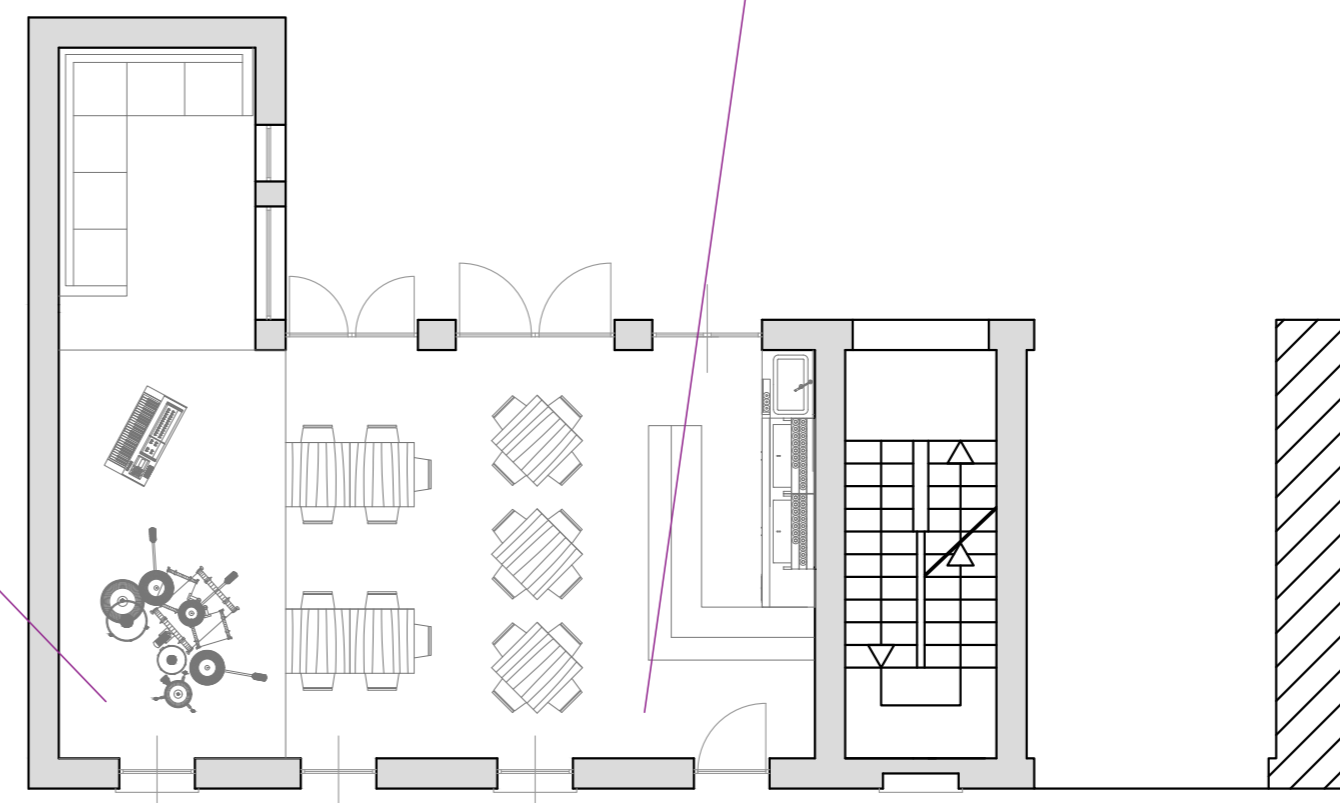
Piano terra
